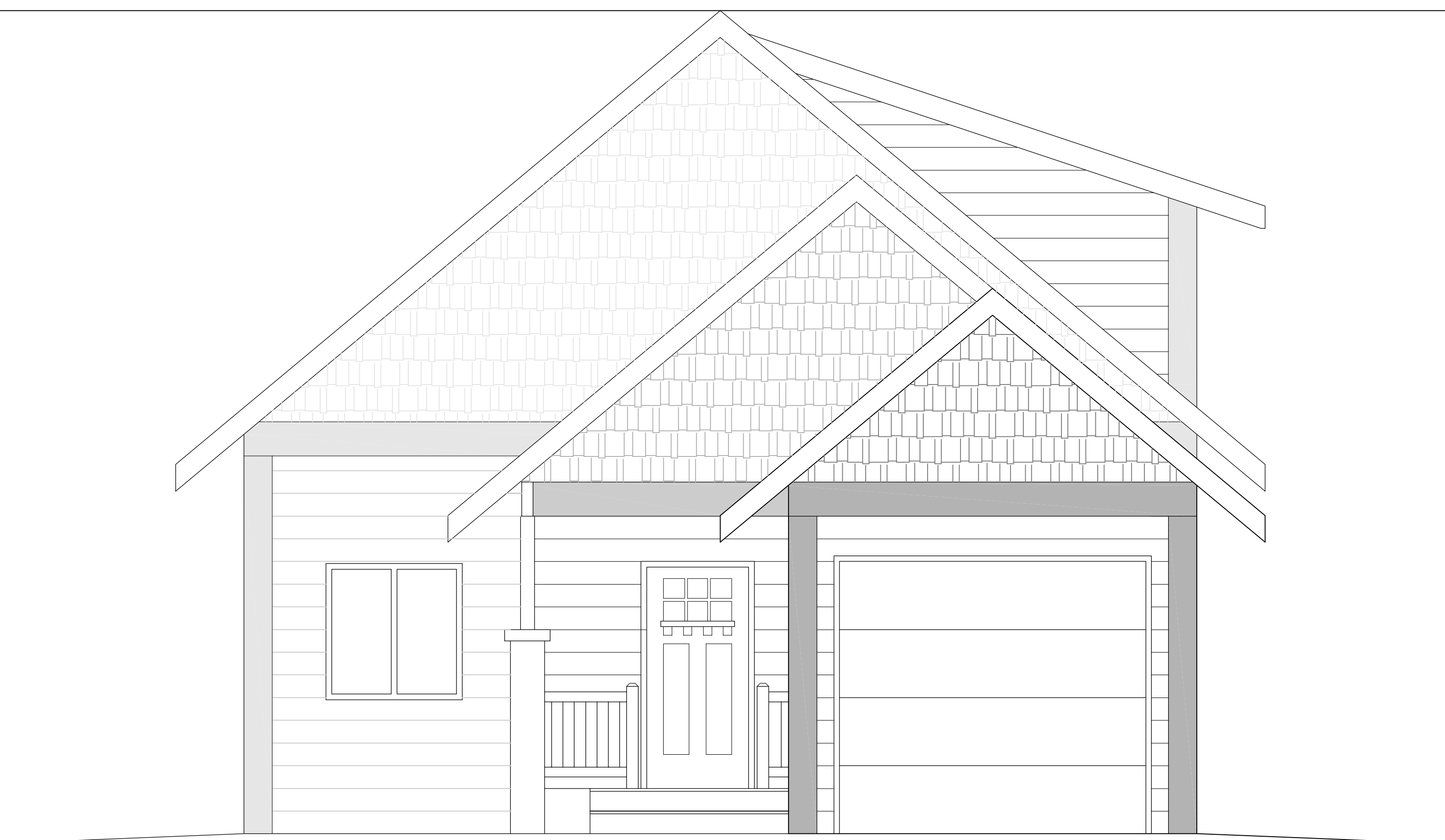
REAR ELEVATION
